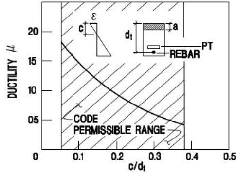
(b) DUCTILITY AND REINFORCEMENT
